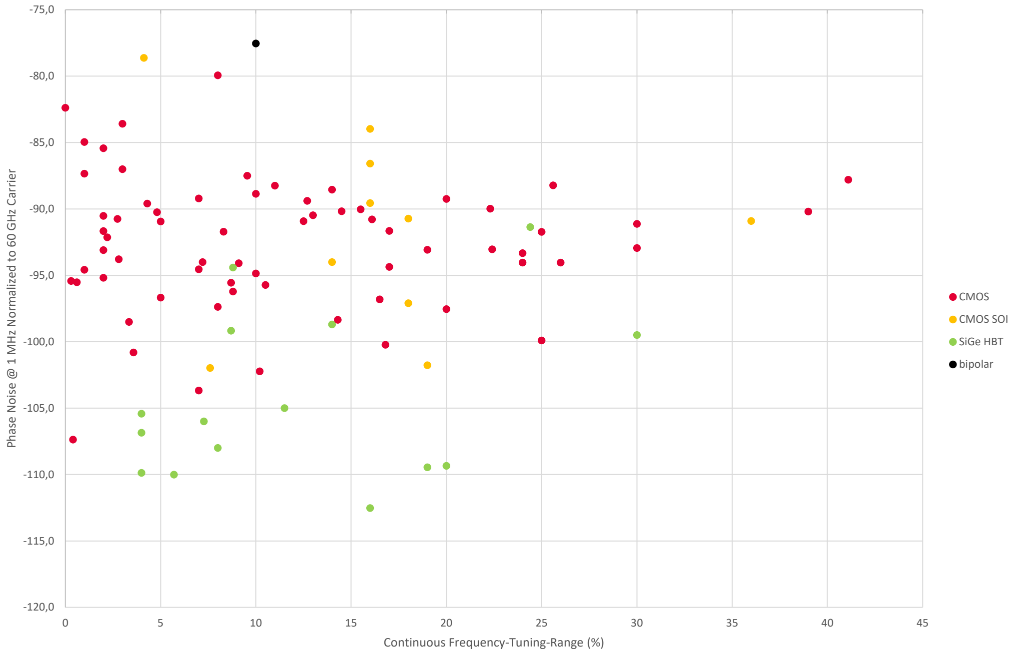
Phase Noise versus Continuous Frequency-Tuning-Range
